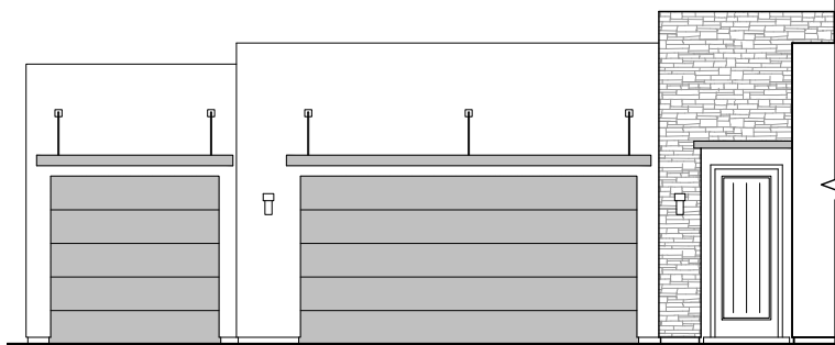
3 Car Garage H Elevation
