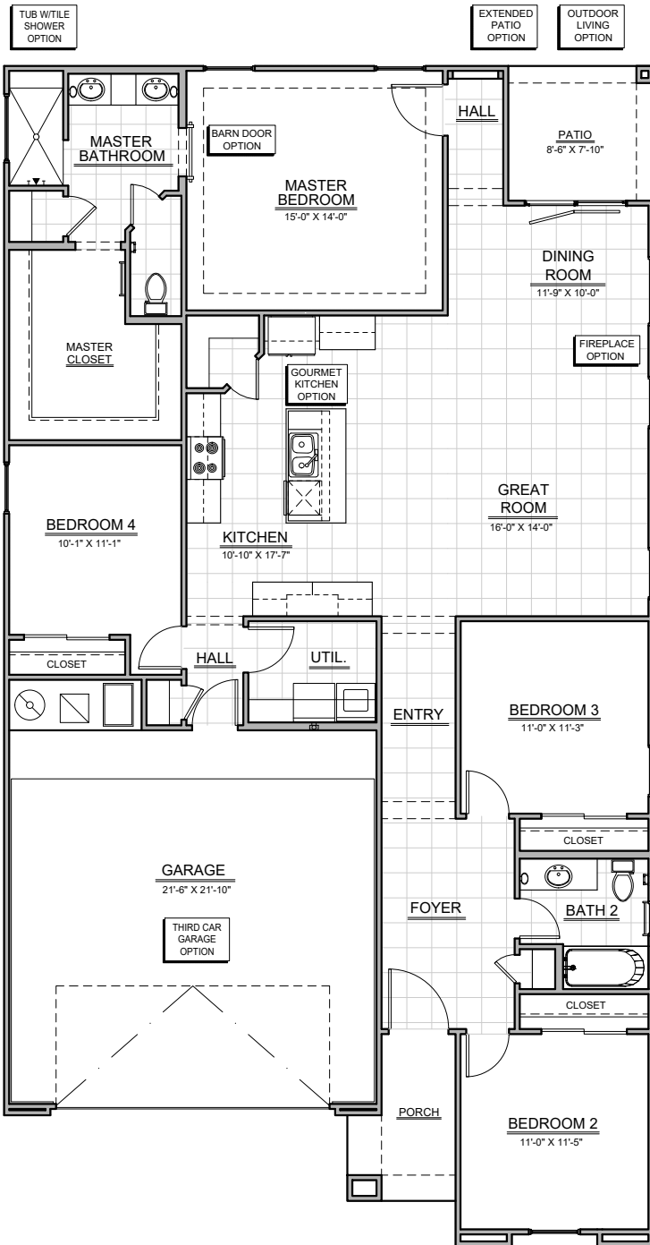
Floor Plan
